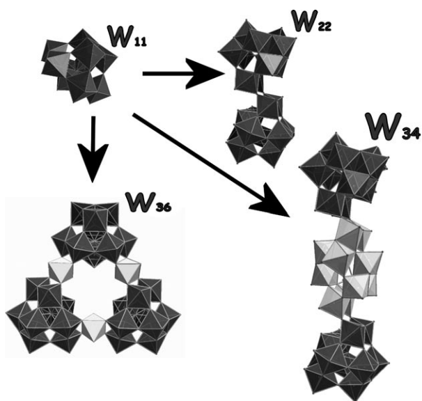
Figure 4. The assembly of the S-shaped \{W_{22}\} and the §-shaped \{W_{34}\} and the trimeric \{W_{36}\} units [19] with the tungsten centers shown as polyhedral representations. The \{W_{11}\} units are shown in dark gray and the \{W_1\} and \{W_{12}\} linkers are shown in light gray.
